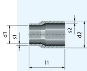
Coaxial Terminator
